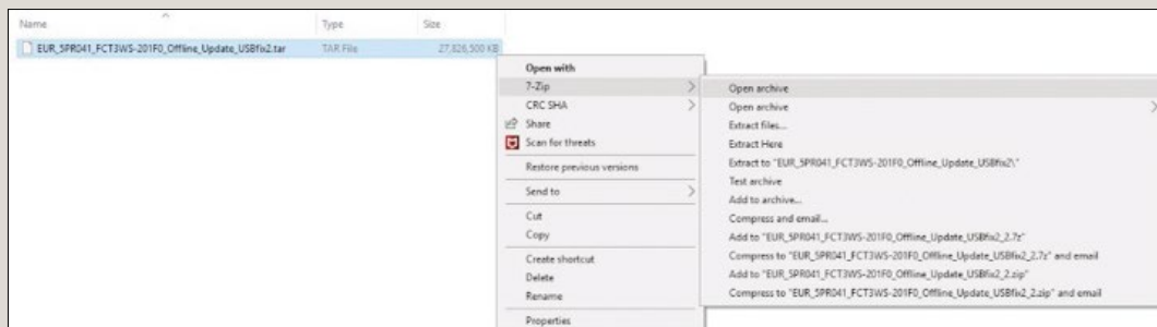
Fig.2 Unzipping path.
